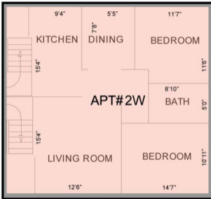
2ND FLOOR
